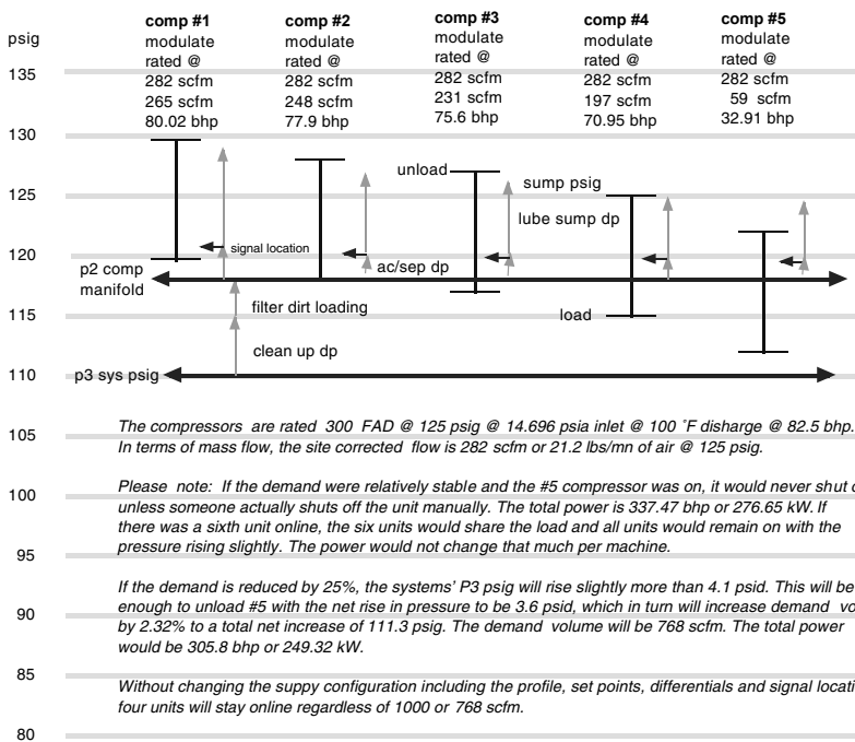
Illustration #2: A 25% Demand Reduction Only Equated to a 10% Power Reduction
