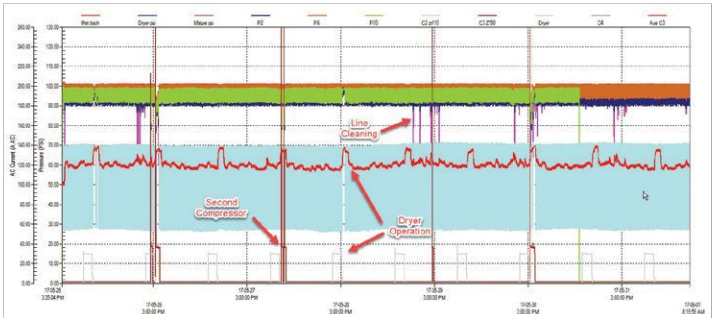
Figure 4: A typical baseline period shows the effects of dryer cooling purge.
