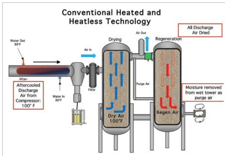
Figure 2 describes the basic drying process for these types of dryers. It is not meant to evaluate one or the other type of dryer. In all cases, proper application and selection requires much more in-depth information.
