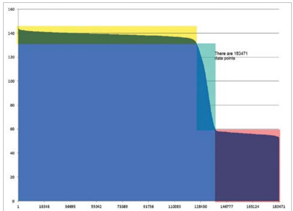
Figure 7: The load duration profile on the original air compressor power input shows areas of possible savings.
