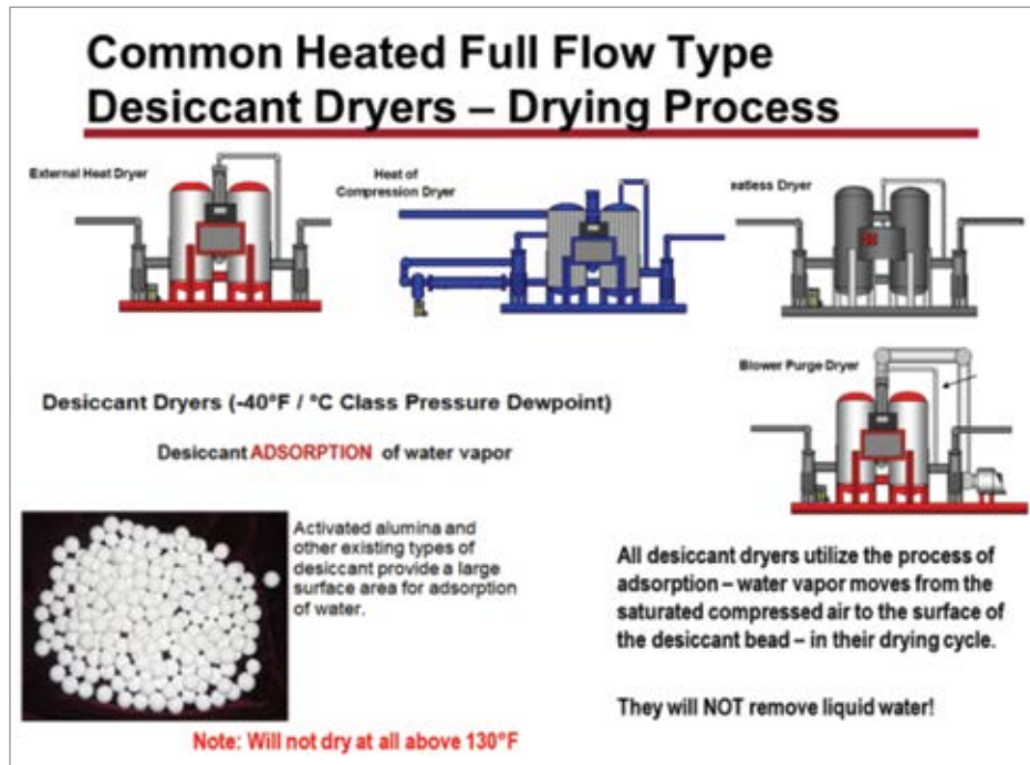
Figure 1. Four common types of twin tower desiccant dryers, and the activated alumina absorption process.
