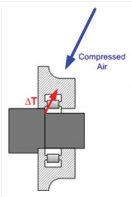
Figure 1: Bearing housing
