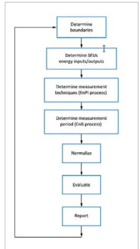
Figure 2: The standard provides definitions and recommended actions on how to determine an energy baseline. (Source CSA C837-16)
