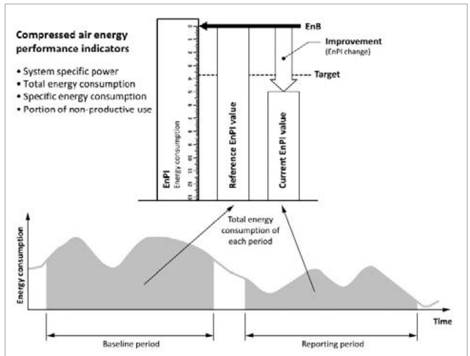
Figure 1: The standard defines a number of Energy Performance Indicators (EnPI's) and guides the reader how to compare a specified baseline period with any reporting period (Source CSA C837-16).
