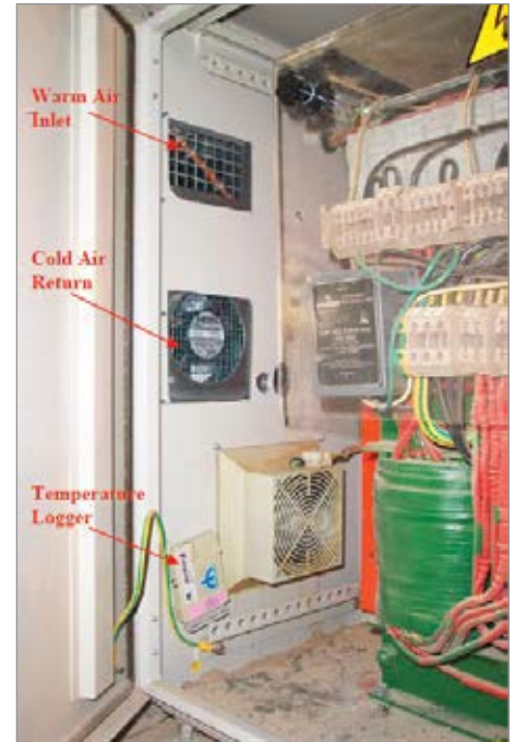
Figure 3: The refrigerated coolers provide some isolation from ambient dust and a good circulation flow inside the cabinet.
