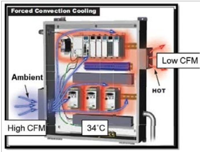
Figure 4: Proton, An Asian auto producer designed a forced convection cooler than uses ambient air to replace their many compressed air powered cabinet coolers (Used with permission).
