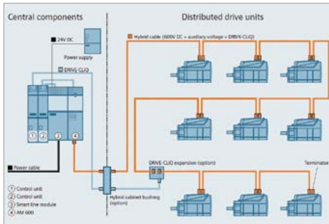
This schematic shows a typical distributed drive application, where all inverter power modules are mounted directly onto the driven axis of the appropriate motor in the machine.
