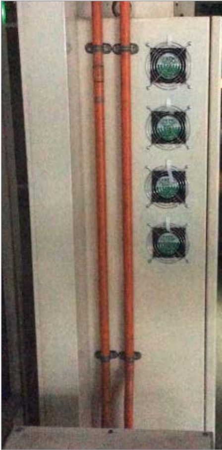
Figure 5: Donut fans provide an adequate flow of cooling air for most panels. Where more cooling is required refrigerated coolers are used.
