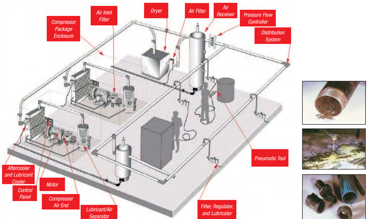
Figure 9. Represents a factory air system. A typical system consists of compressor(s), controls and regulators, dryer, receiver, ring main and individual users. The photographs on the right indicate corrosion and build-up from improper filter maintenance, costly and corrosive condensation from a poorly maintained dryer, and damaged tools and fittings, all of which can lead to unscheduled maintenance increased costs and inefficiencies. Source: www.energymanagertraining.com/equipment_all/compressors/1.htm
